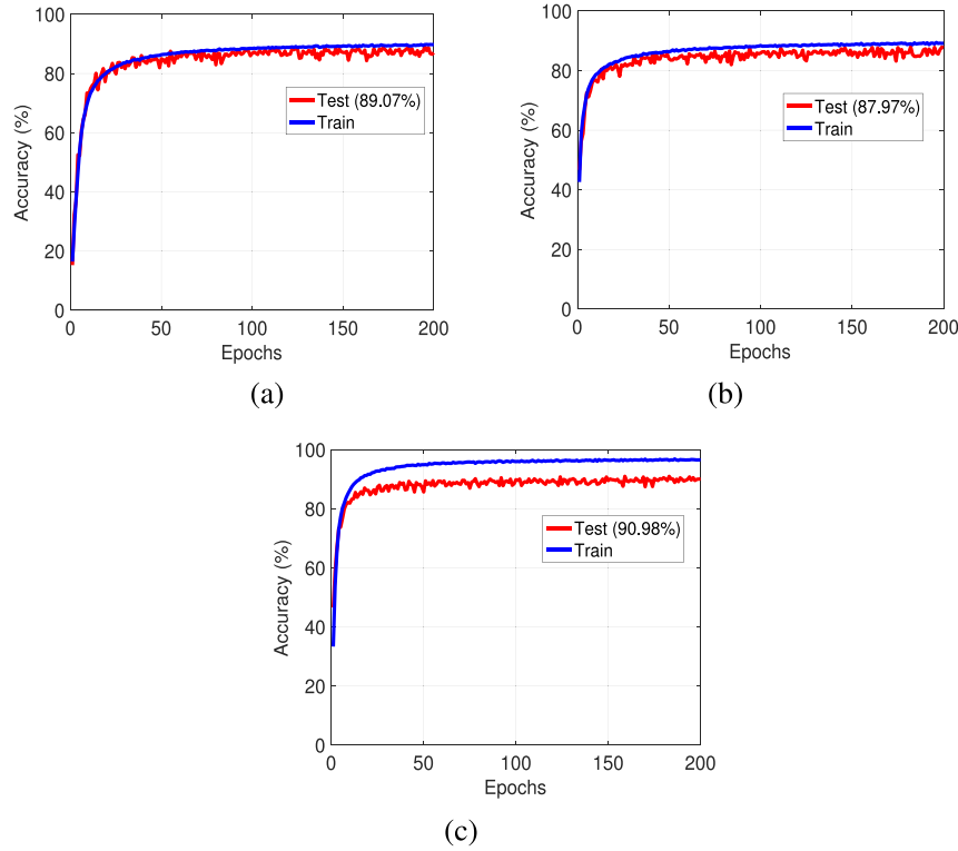
Fig. 3. Training curves corresponding to three different models with softmax on CIFAR-10 dataset. Curve for model A is represented in (a). (b) shows the plot for model B and (c) represents the plot for model C. Train and test accuracies are represented by blue and red curves respectively. (For interpretation of the references to color in this figure legend, the reader is referred to the web version of this article.)
