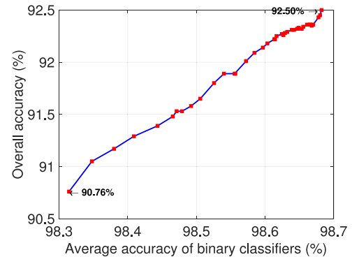
Fig. 5. Relationship between the performance of binary classifiers and overall solution when fine-tuning using triplet loss with base model A. The red points correspond to every 100th iteration. (For interpretation of the references to color in this figure, the reader is referred to the web version of this article.)
