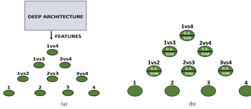
Fig. 1. Two variants of multiclass classification using binary classifiers arranged in a DAG structure. (a) shows the architecture of the model for a 4-class problem where features learned by the deep network are used to train all the classifiers. Here each node is a binary classifier for a pair of classes. In (b), the architecture for the same 4-class is shown but here each node represents a combination of the deep architecture (D.A.) and the Support Vector Machine (SVM) classifier. This makes it possible to learn more pairwise discriminative features to further improve the performance of the classifiers.
