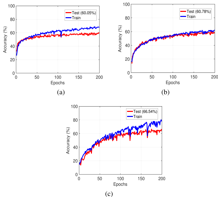
Fig. 6. Training curves corresponding to three different models with softmax on STL-10 dataset. Curve for model S1 is represented in (a). (b) shows the plot for model S2 and (c) represents the plot for model L1. Train and test accuracies are represented by blue and red curves respectively. (For interpretation of the references to color in this figure legend, the reader is referred to the web version of this article.)
