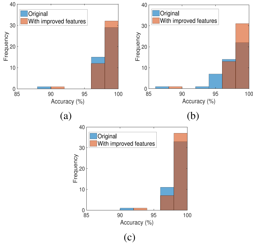
Fig. 4. Histogram plots of test accuracies of the individual binary classifiers in the DAG before (Original) and after fine-tuning the base model A, B and C are shown in (a), (b) and (c) respectively. (For interpretation of the references to color in this figure legend, the reader is referred to the web version of this article.)
