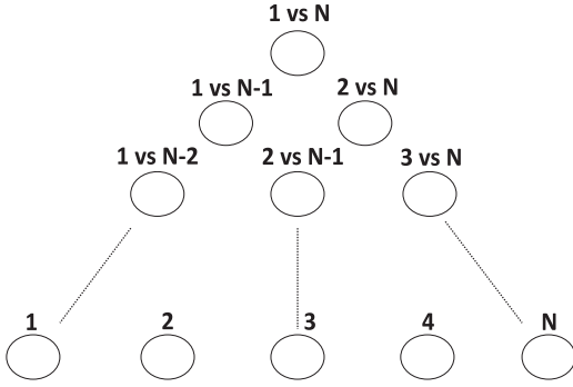
Fig. 2. Arrangement of the different binary classifiers in the DAG for a N -class problem.
